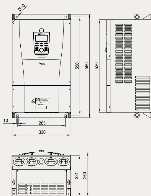
N700-300LF/300HF
