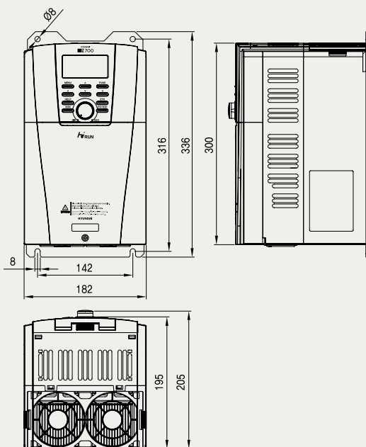
N700-055LF/055HF, N700-075LF/075HF N700-110LF/110HF
