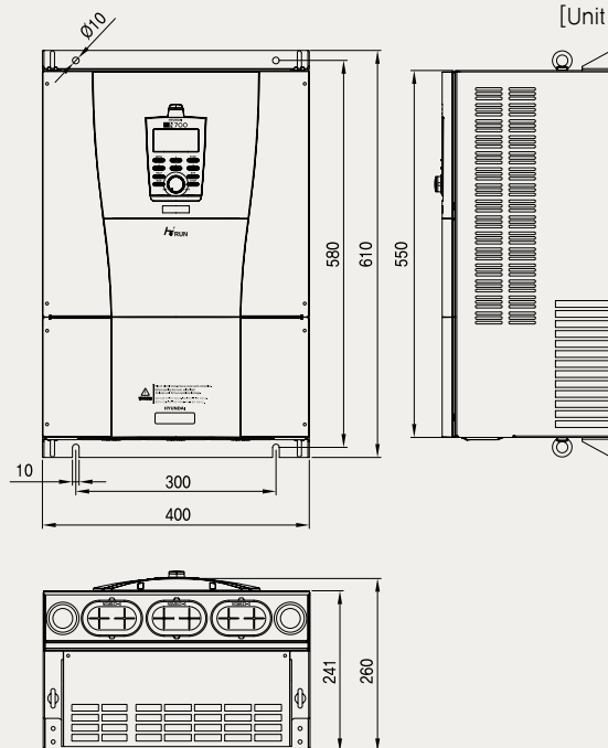
N700-370LF/370HF, N700-450LF/450HF
