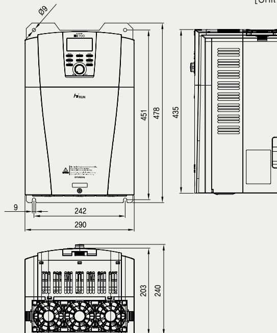
N700-150LF/150HF, N700-185LF/185HF N700-220LF/220HF
